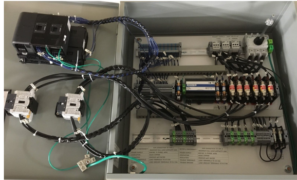
Figure 3 on right - Dual pump controller with HMI for large pumping skid (Inside)
