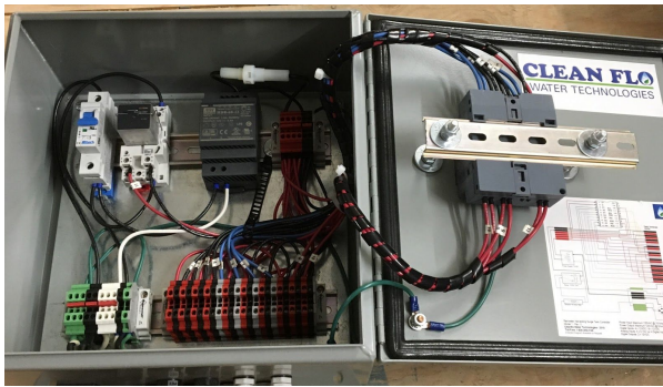
Figure 1 to left - Rainwater Pump Controller
